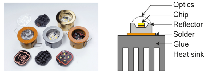
Fig. 2: High performance LED system based on thermally conductive plastics consisting of Molded Interconnect Device, housing and optics [Courtesy of RF Plast GmbH and Dommel GmbH]
