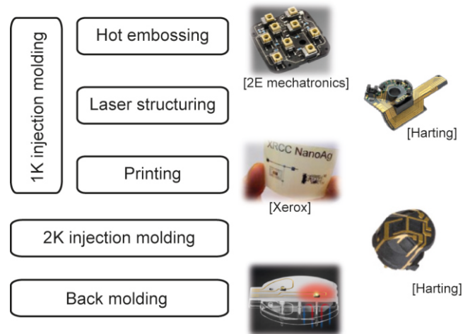
Fig. 5: Overview of 3D-MID metallization technologies
