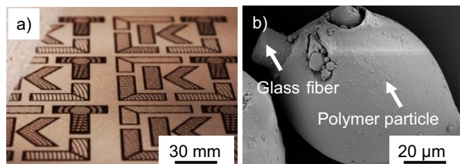
Fig. 6: a) Part fabrication of Polyamide 12 filled with 15 vol.-% copper b) Particle-filled system
